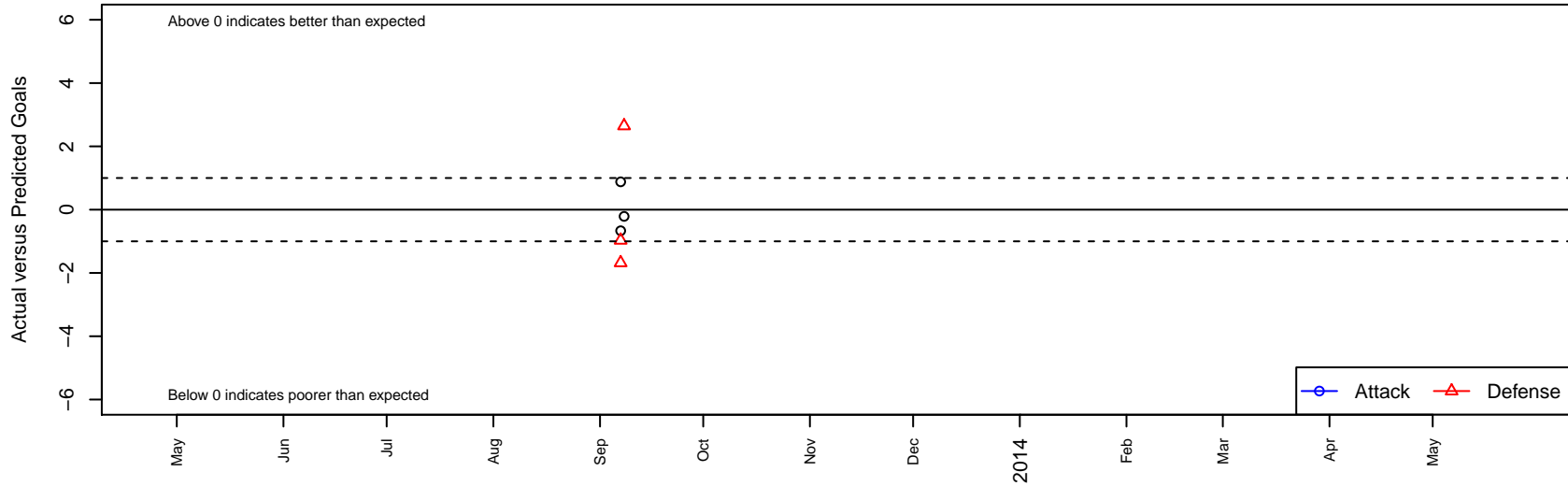
The Academy Cads G01 Dots are actual minus expected GF (blue circles) and GA (red triangles). Blue line is smoothed change in attack strength. Red is smoothed change in defense strength.
